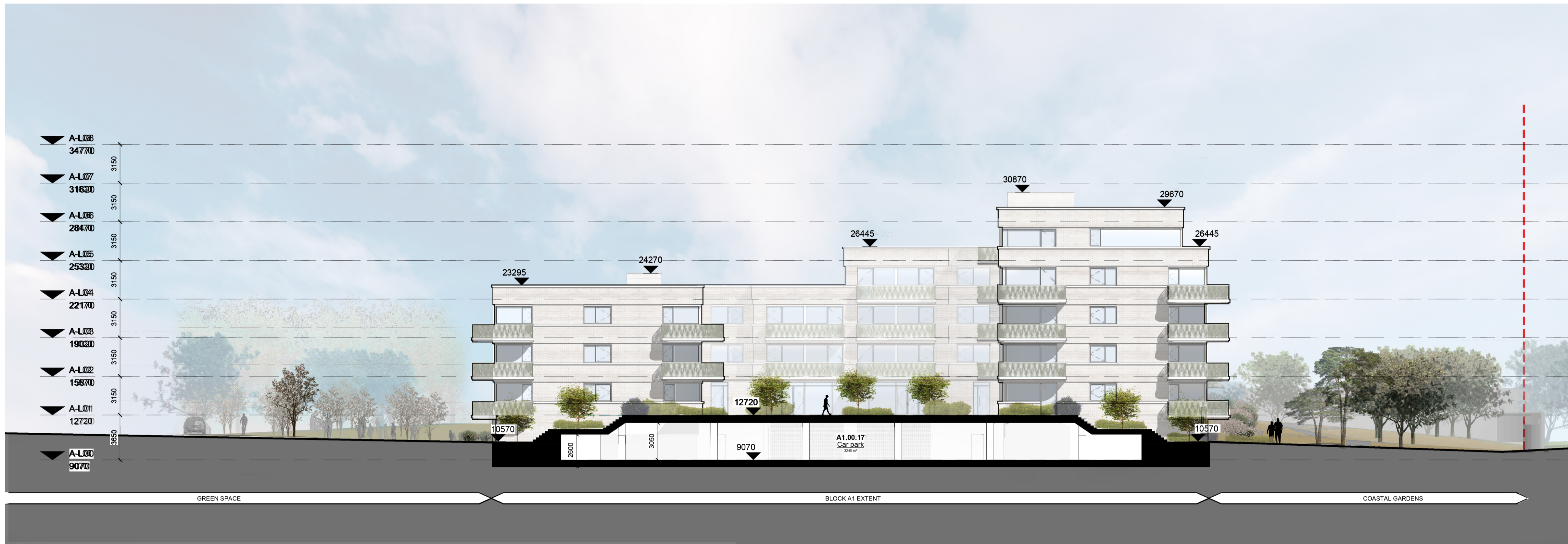
Block A - Section AA 1 : 200
